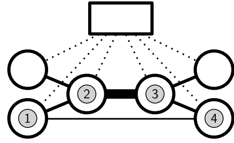
Fig. 2. An example of a computed MST topology where peers with better connections (② and ③) act as supernodes, and with redundancy (① and ④)
