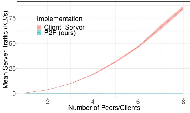
Fig. 3. Mean server network traffic (0.95 confidence interval) against number of clients/peers for a traditional client-server model versus our optimised P2P version
