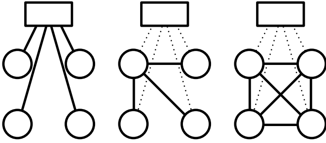
Fig. 1. Three networking topologies of interest between servers (rectangles) and peers/clients (circles) – client-server model (left), hosted P2P (middle), and full P2P (right)
